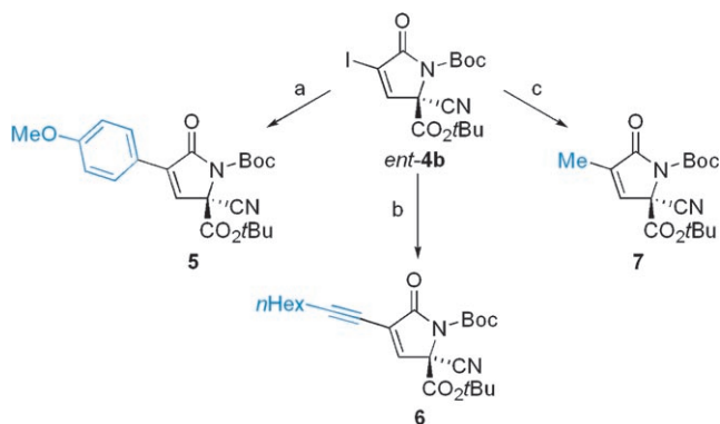
Scheme 4. Different cross-coupling reactions with ent-4b . Reagents and conditions: a) 10% [Pd(PPh 3 ) 4 ], PMP-B(OH) 2 , toluene, 2 M aq Na 2 CO 3 , 60 °C, 75 min, 71 %; b) 10% [PdCl 2 (PPh 3 ) 2 ], 15 % CuI, 1-octyne, DIPEA, CH 2 Cl 2 , RT, 40 min, 83 %; c) 5 % [PdCl 2 (PPh 3 ) 2 ], ZnMe 2 , DMF/THF (1:1), RT, 105 min, 86 %. DMF = N,N -dimethylformamide, PMP = para -methoxyphenyl, DIPEA = N,N -diisopropylethylamine.
